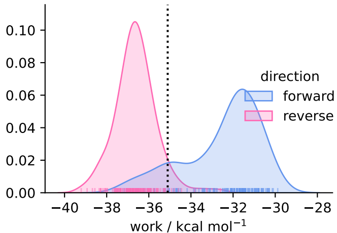
solvent ( N = 147 )
