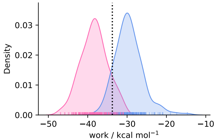
complex ( N = 178 )
