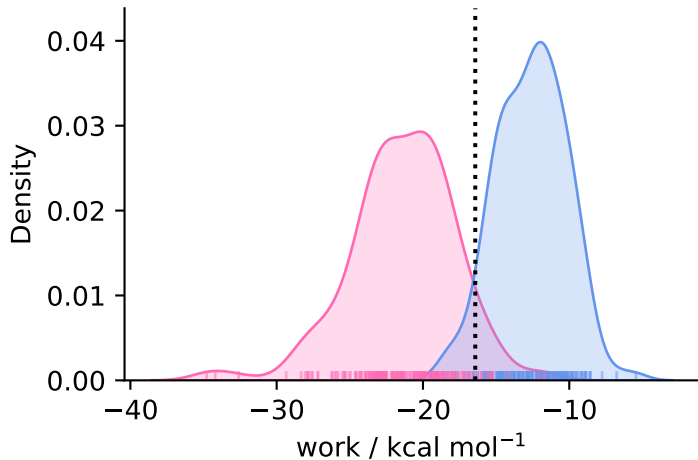
complex ( N = 176 )
