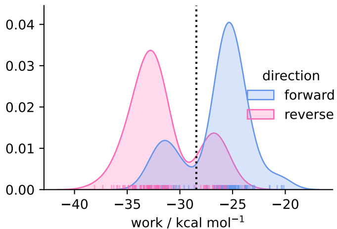
solvent ( N = 126 )
