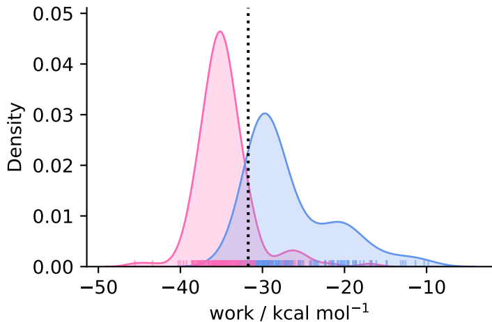
complex ( N = 176 )
