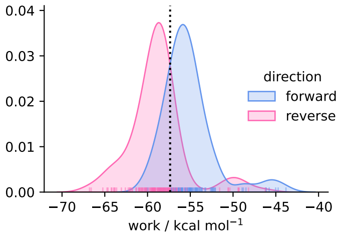
solvent ( N = 130 )
