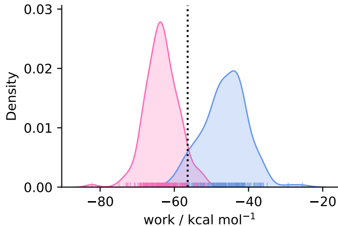
complex ( N = 178 )
