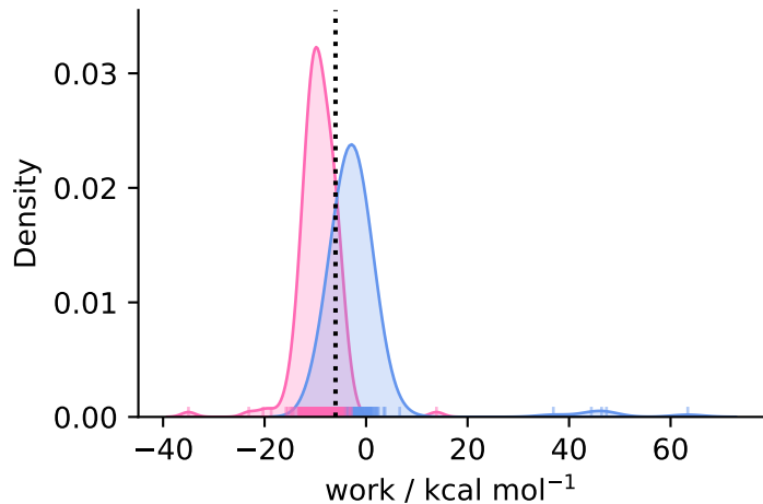
complex ( N = 178 )
