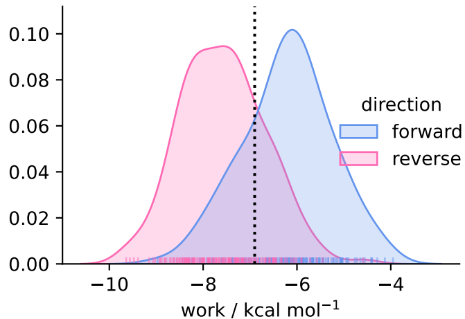
solvent ( N = 160 )
