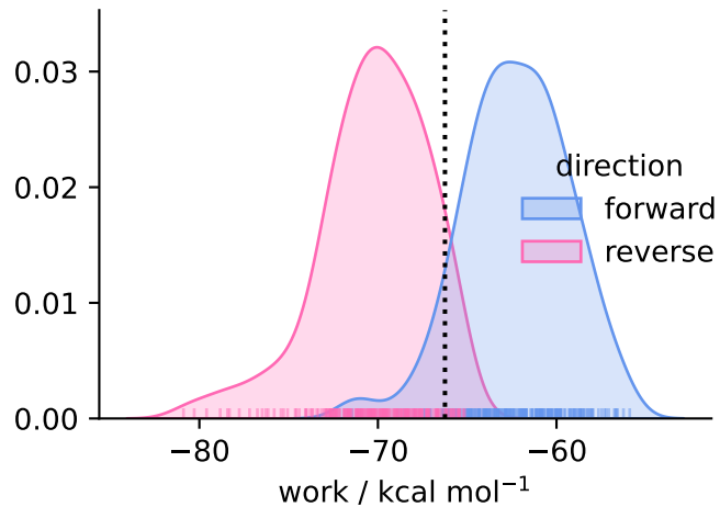
solvent ( N = 212 )
