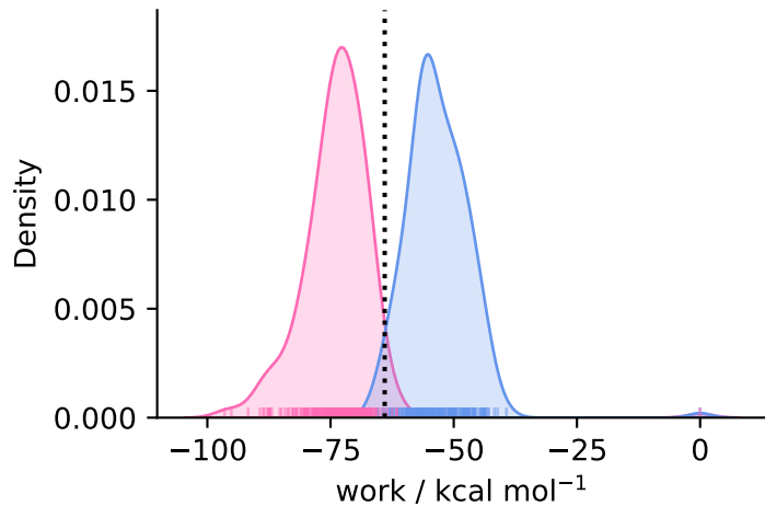
complex ( N = 215 )
