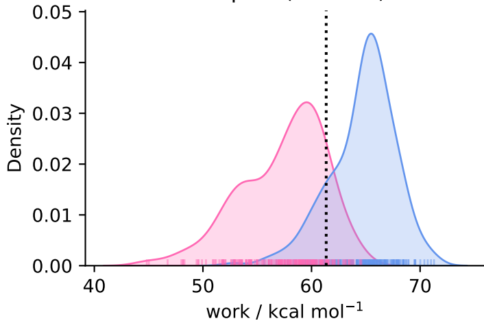
complex ( N = 223 )
