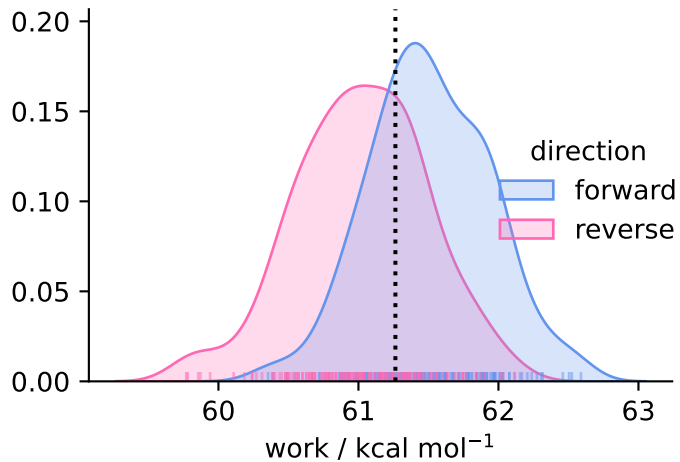
solvent ( N = 163 )
