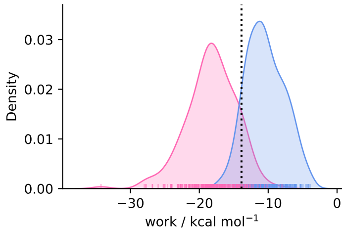
complex ( N = 222 )
