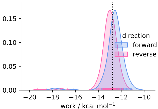
solvent ( N = 217 )
