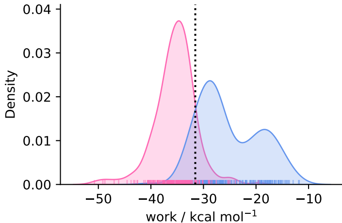
complex ( N = 224 )
