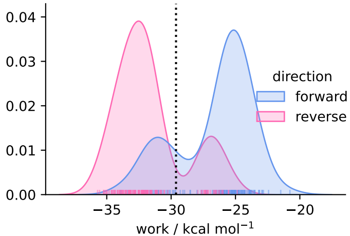
solvent ( N = 145 )
