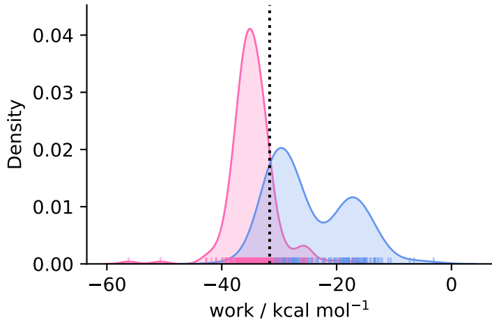
complex ( N = 214 )
