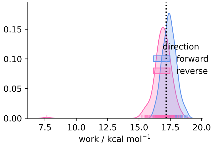
solvent ( N = 216 )
