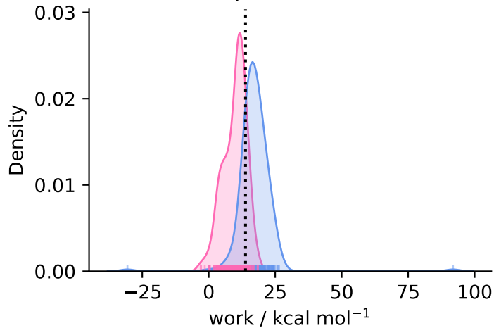
complex ( N = 208 )
