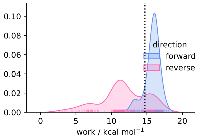
solvent ( N = 172 )
