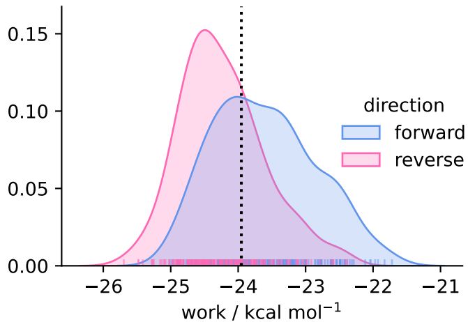
solvent ( N = 201 )
