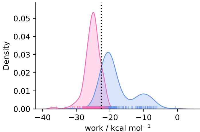
complex ( N = 230 )
