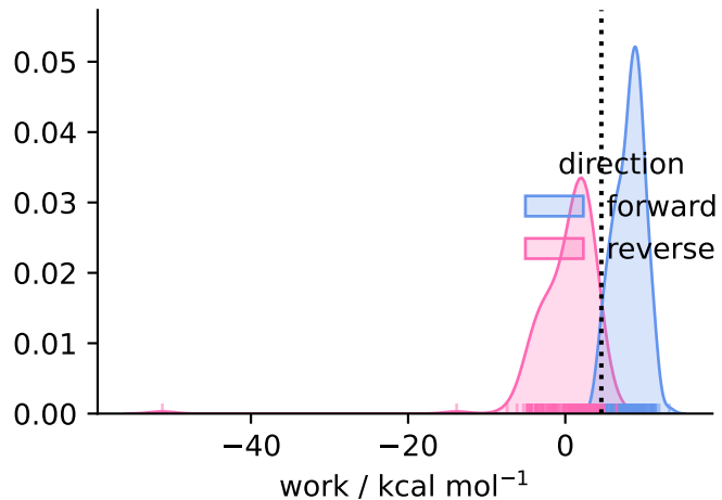
solvent ( N = 216 )
