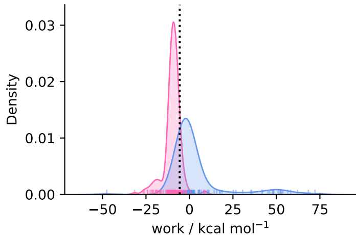
complex ( N = 219 )
