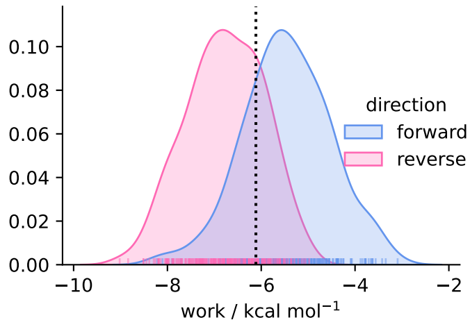
solvent ( N = 227 )
