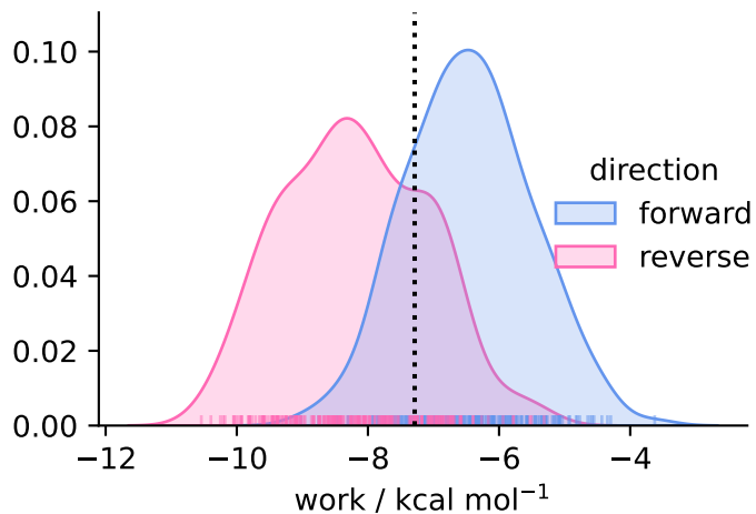
solvent ( N = 221 )
