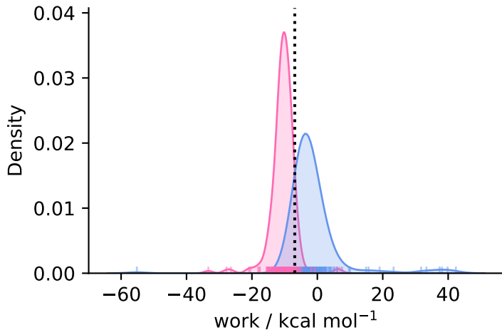
complex ( N = 214 )
