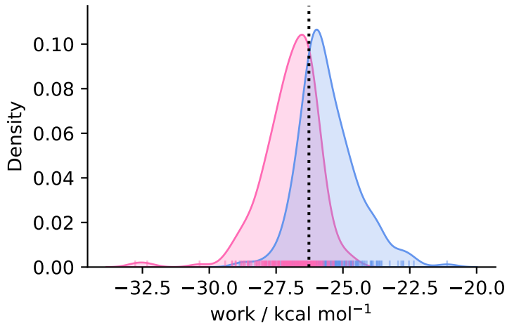
complex ( N = 214 )
