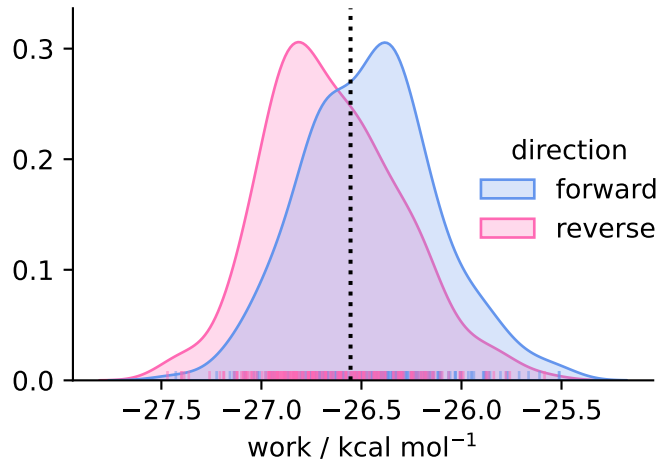
solvent ( N = 230 )
