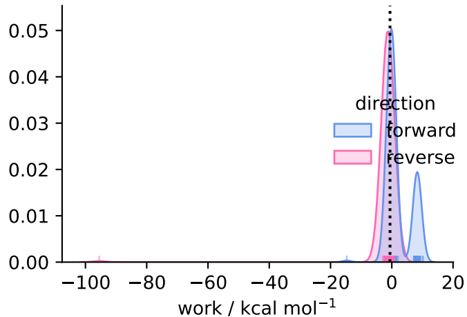
solvent ( N = 231 )
