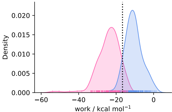
complex ( N = 194 )
