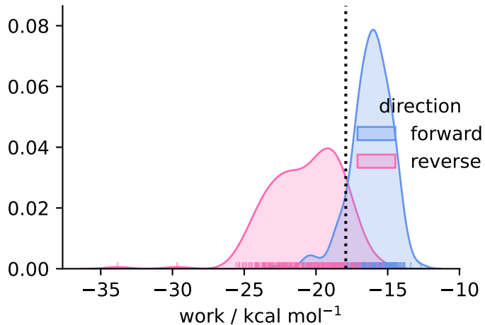
solvent ( N = 218 )
