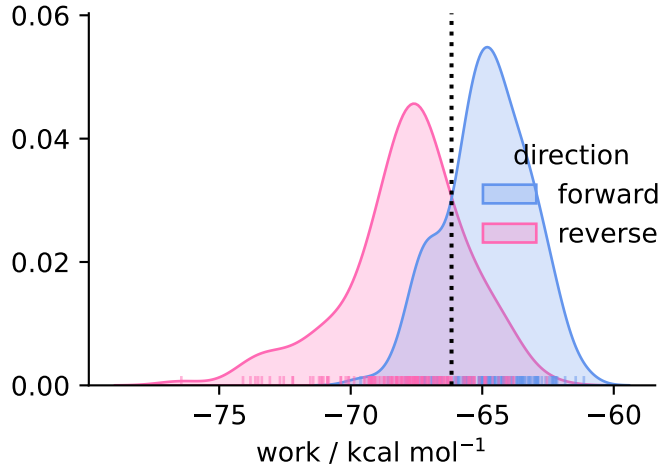
solvent ( N = 158 )
