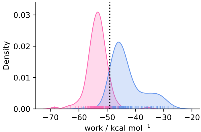
complex ( N = 140 )
