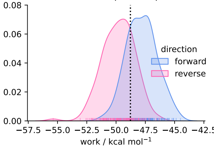
solvent ( N = 159 )
