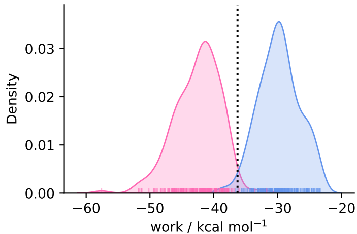
complex ( N = 199 )
