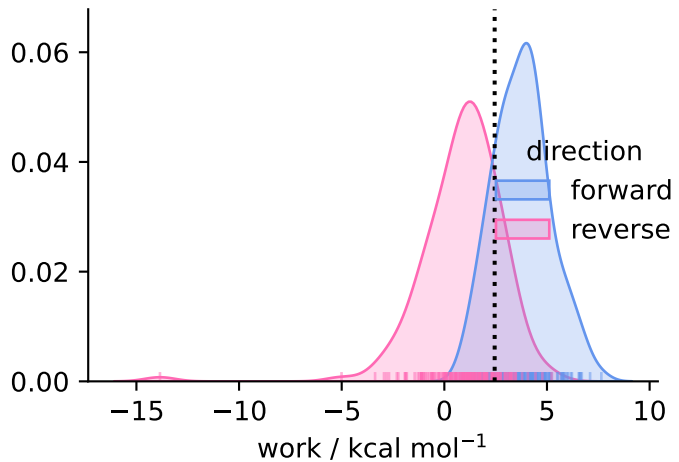
solvent ( N = 158 )
