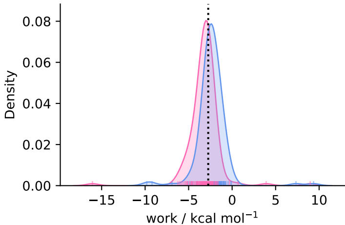
complex ( N = 132 )
