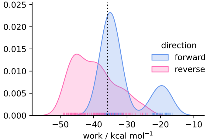
solvent ( N = 154 )
