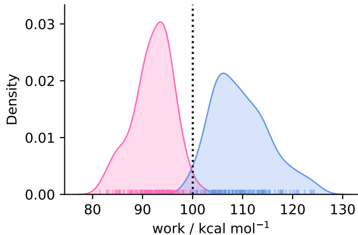
complex ( N = 153 )
