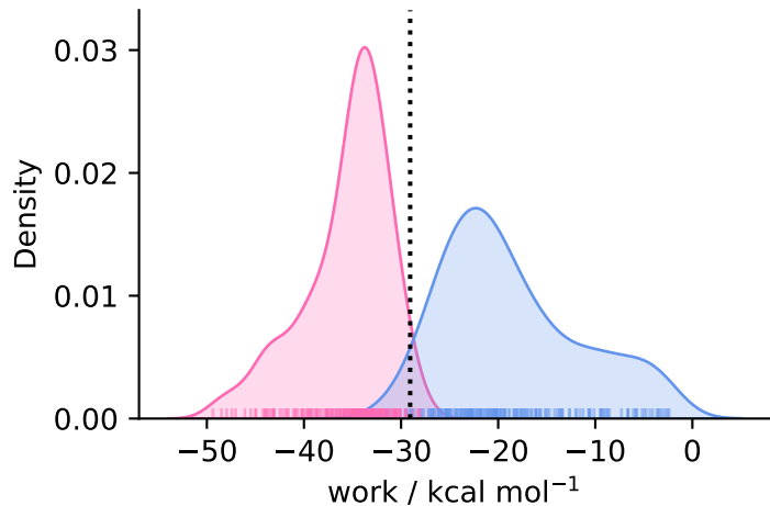
complex ( N = 188 )
