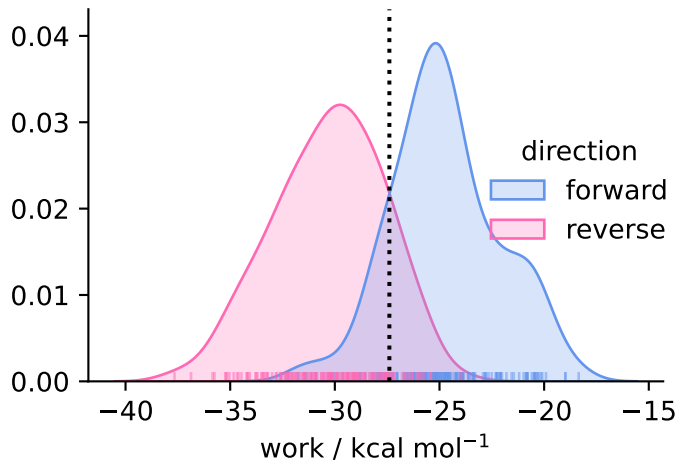
solvent ( N = 159 )
