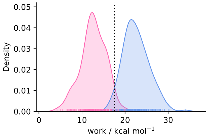
complex ( N = 200 )
