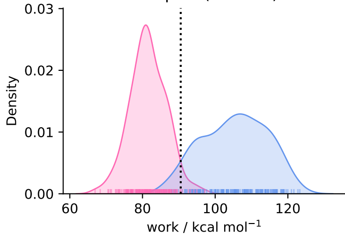
complex ( N = 196 )
