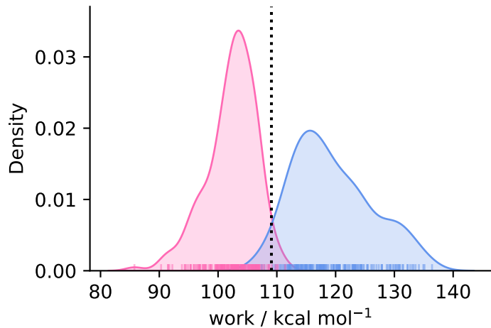
complex ( N = 183 )
