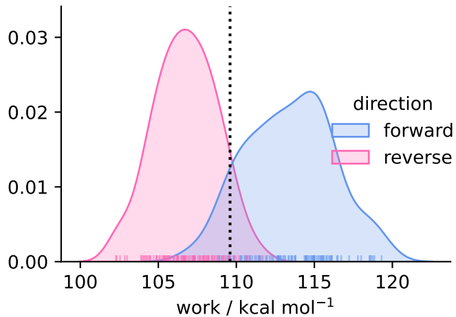
solvent ( N = 99 )
