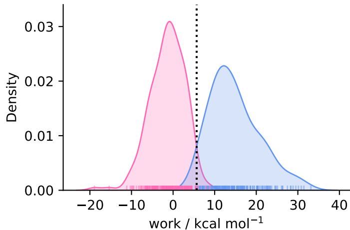
complex ( N = 194 )
