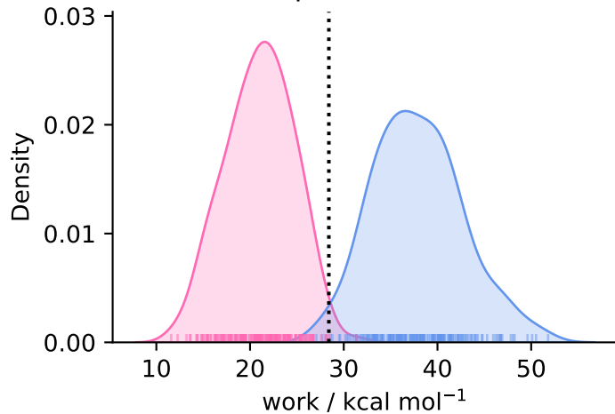
complex ( N = 200 )
