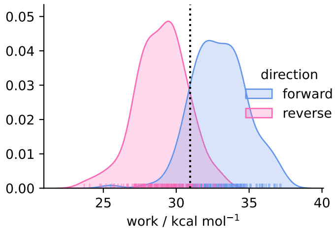
solvent ( N = 160 )
