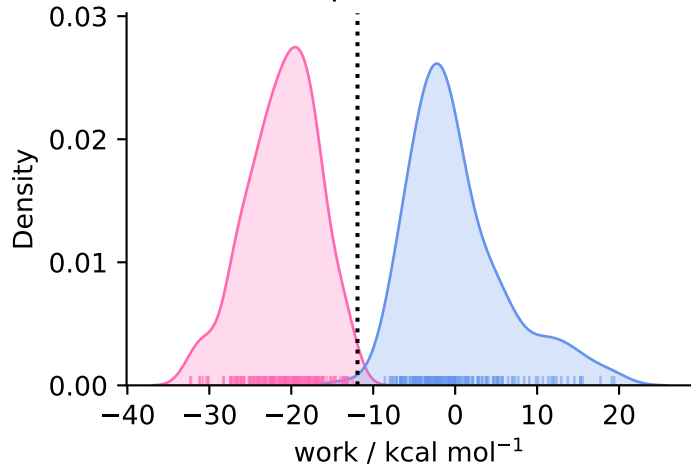
complex ( N = 169 )
