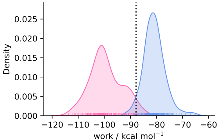
complex ( N = 160 )
