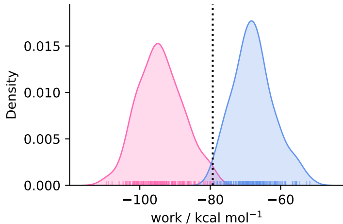
complex ( N = 161 )
