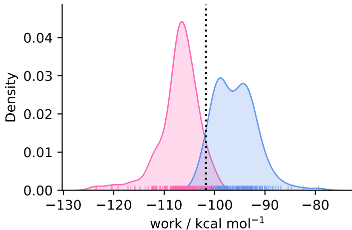
complex ( N = 200 )
