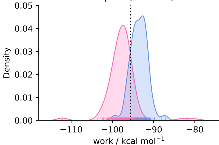
complex ( N = 159 )
