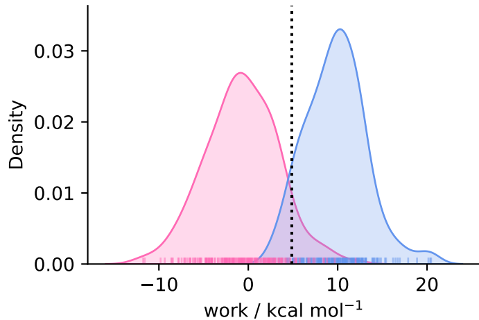
complex ( N = 200 )
