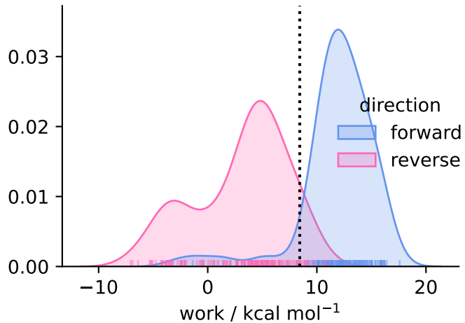
solvent ( N = 159 )
