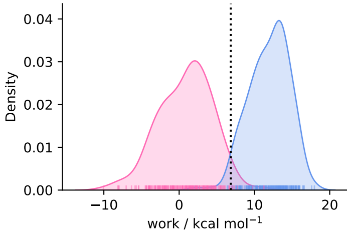
complex ( N = 199 )
