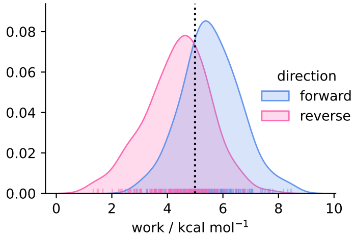
solvent ( N = 160 )
