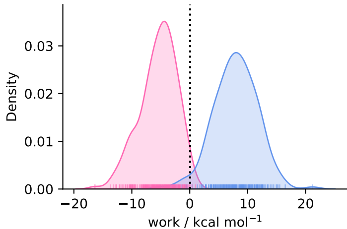
complex ( N = 197 )
