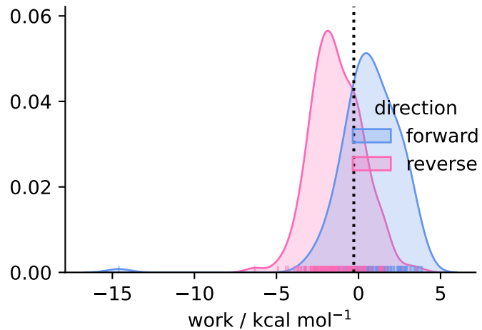
solvent ( N = 159 )
