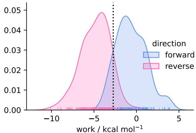
solvent ( N = 159 )
