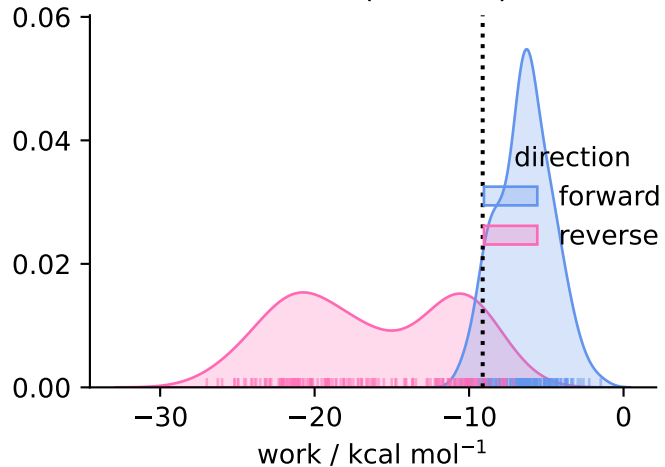
solvent ( N = 160 )
