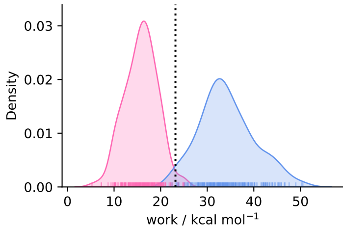
complex ( N = 200 )
