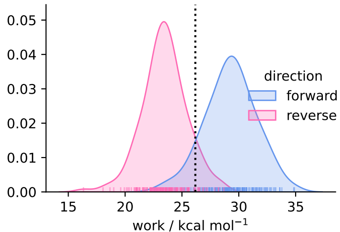
solvent ( N = 160 )
