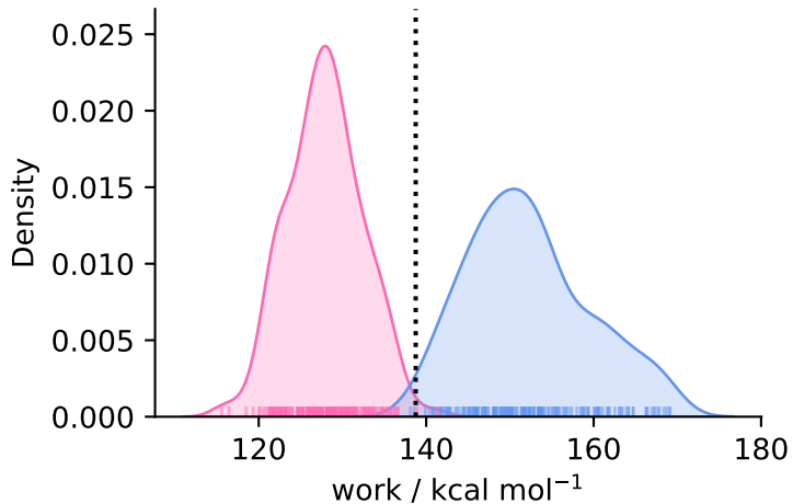
complex ( N = 191 )
