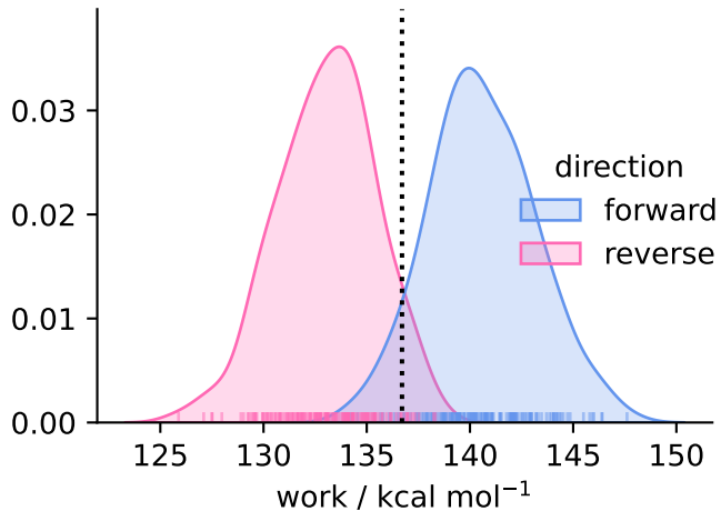
solvent ( N = 160 )
