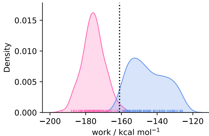
complex ( N = 149 )
