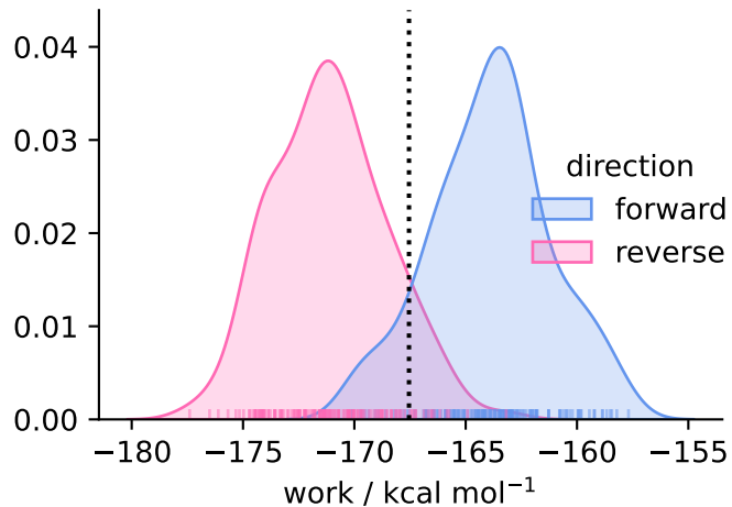
solvent ( N = 153 )
