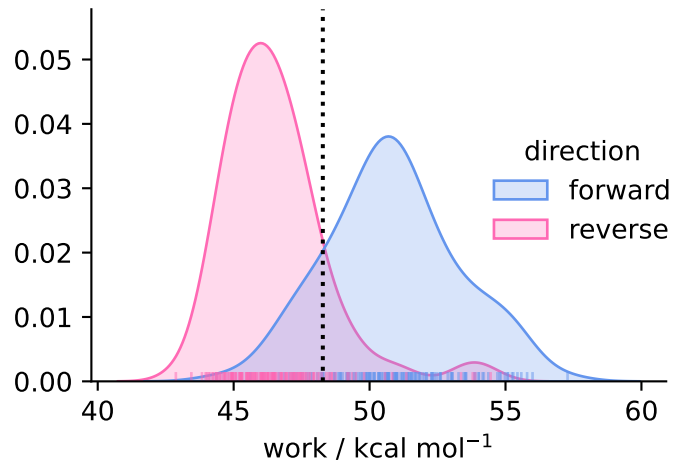
solvent ( N = 147 )
