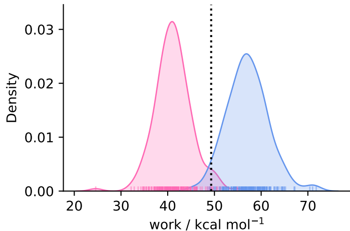
complex ( N = 185 )
