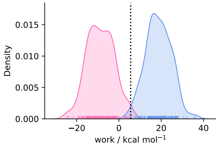
complex ( N = 187 )
