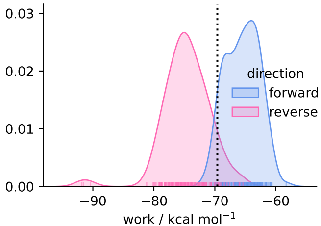
solvent ( N = 158 )
