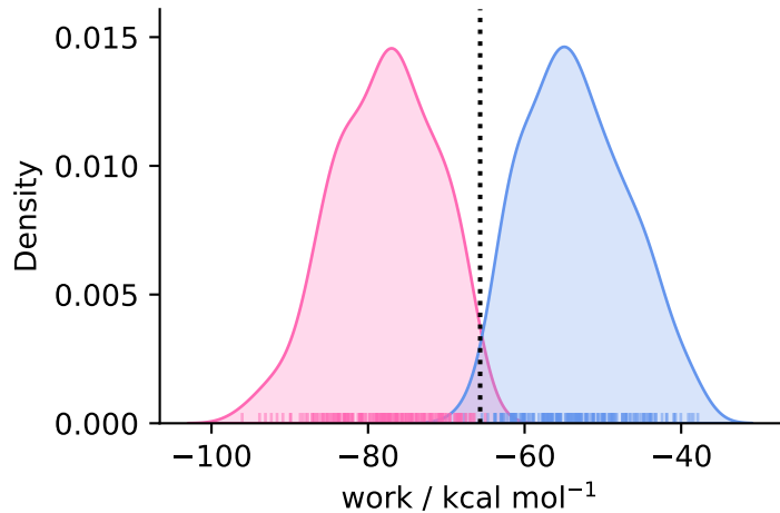
complex ( N = 180 )
