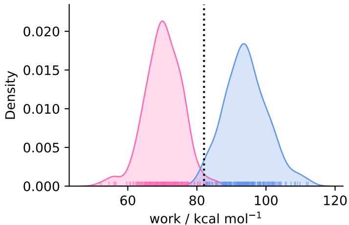
complex ( N = 193 )
