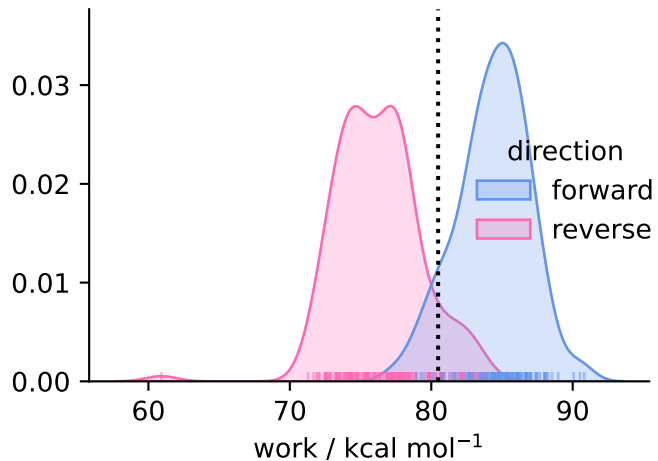
solvent ( N = 153 )
