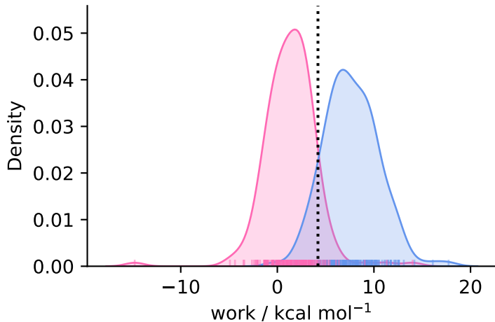
complex ( N = 168 )
